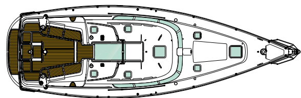
Plan de pont / Deck layout / Deckplan
