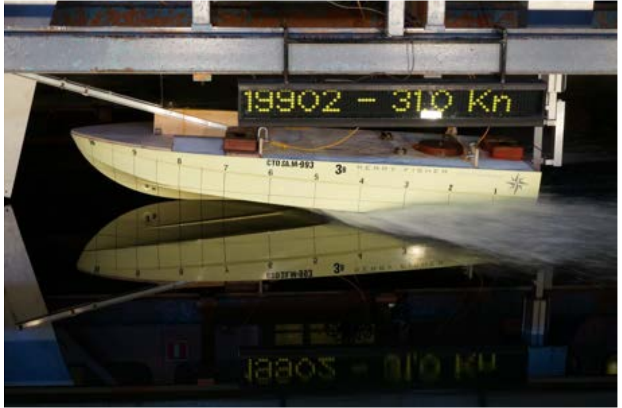
NEW HULL OPTIMIZED FOR OUTBOARDS AND FLAT CRUISING AT INTERMEDIATE SPEEDS, IN THE SAME SPIRIT AS THE HULL DEVELOPED FOR THE MERRY FISHER 1095.
